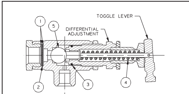
110832 Series Pilot Valve (continuous run operation) Add dash # listed below to 110832 (per pressure setting) to obtain correct pilot valve.
