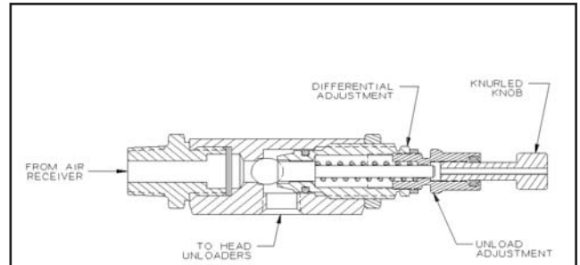
110998 Series Pilot Valve (dual control operation) Add dash # listed below to 110998 (per pressure setting) to obtain correct pilot valve.
